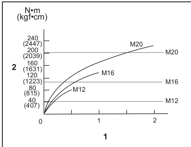
1. Fastening time (second) 2. Fastening torque
