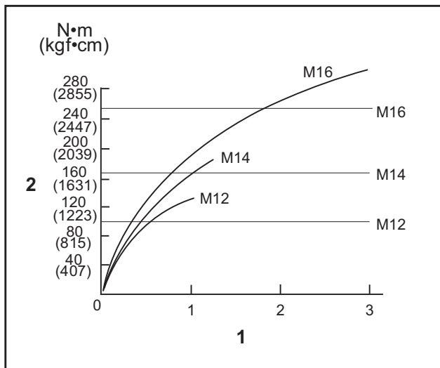
1. Fastening time (second) 2. Fastening torque
